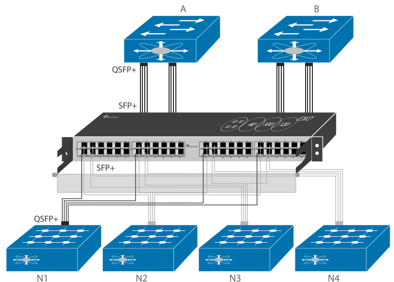
Each SFP+ data lane can be redirected and recombined to QSFP+
